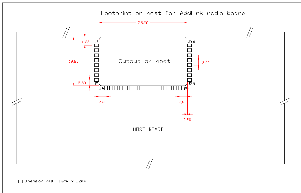
Figure 6-8: Host board cut-out
