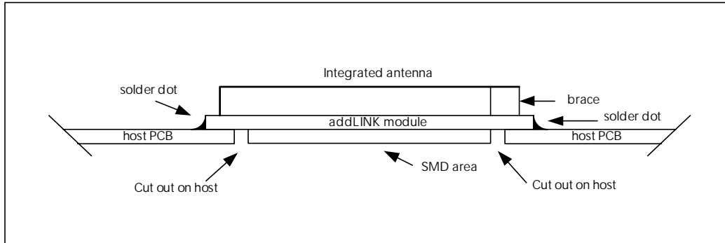
Figure 6-7: addLINK mounting
