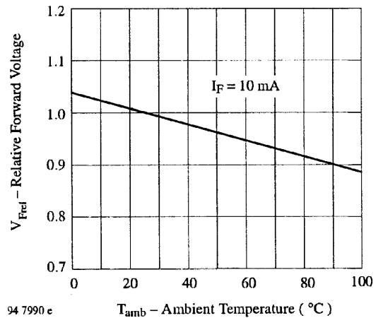
Figure 5. Relative Forward Voltage vs. Ambient Temperature
